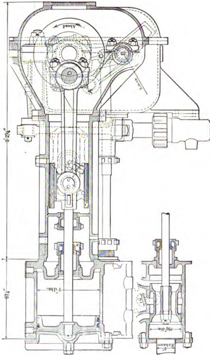
FIG. 276.—Sectional View of the Thornycroft Compound Steam Engine.
